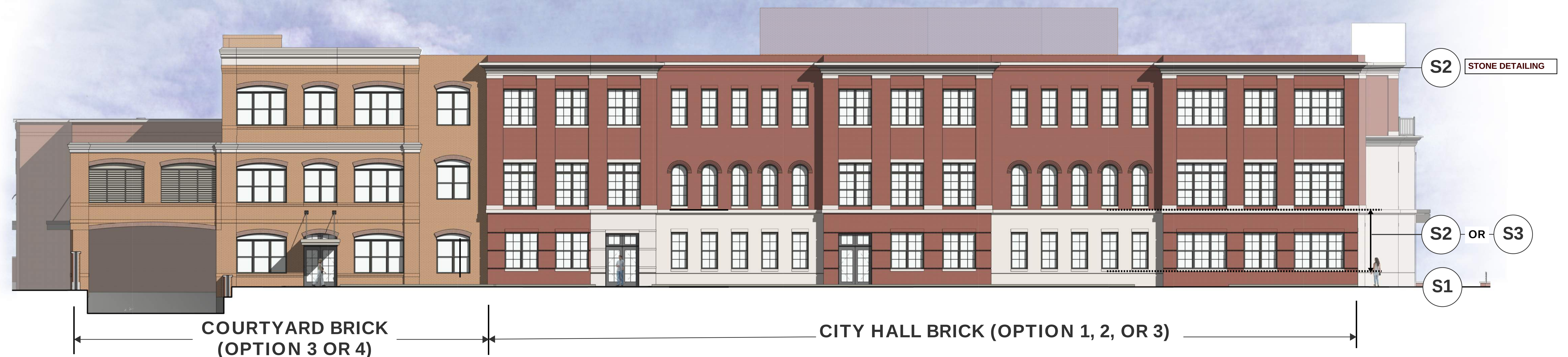
ALLEY ELEVATION
