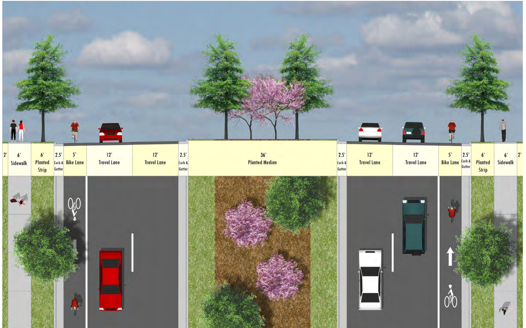
FIGURE 3.22: 4 LANE - 132' SECTION
