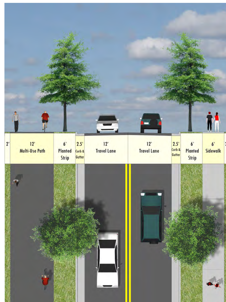
FIGURE 3.15: 2 LANE - 63' SECTION
